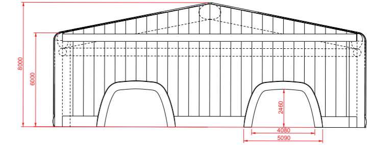
FRONT ELEVATION
