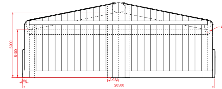
SIDE ELEVATION
