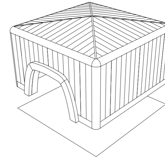
PERSPECTIVE VIEW (WITH GROUND SHEET)
